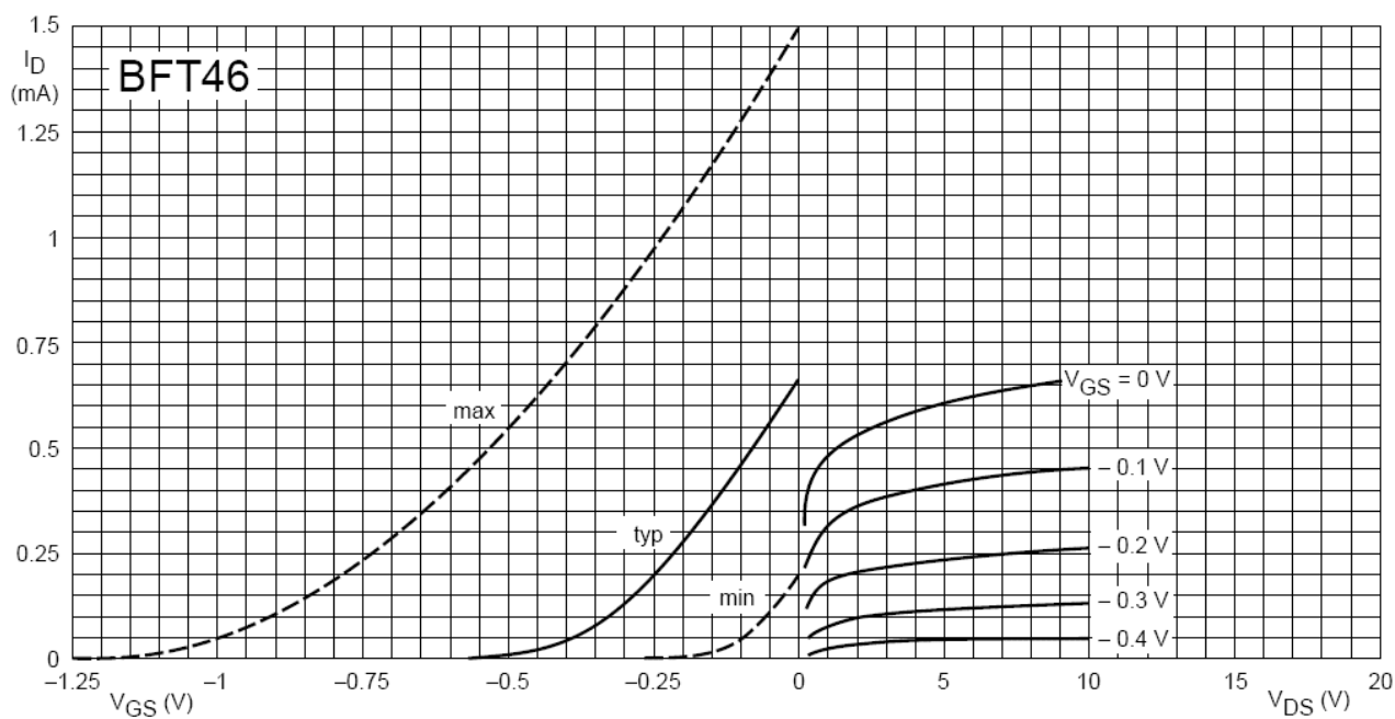
Fig.3 Typical values. V_{DS} = 10\text{ V} ; T_j = 25^\circ\text{C} .
